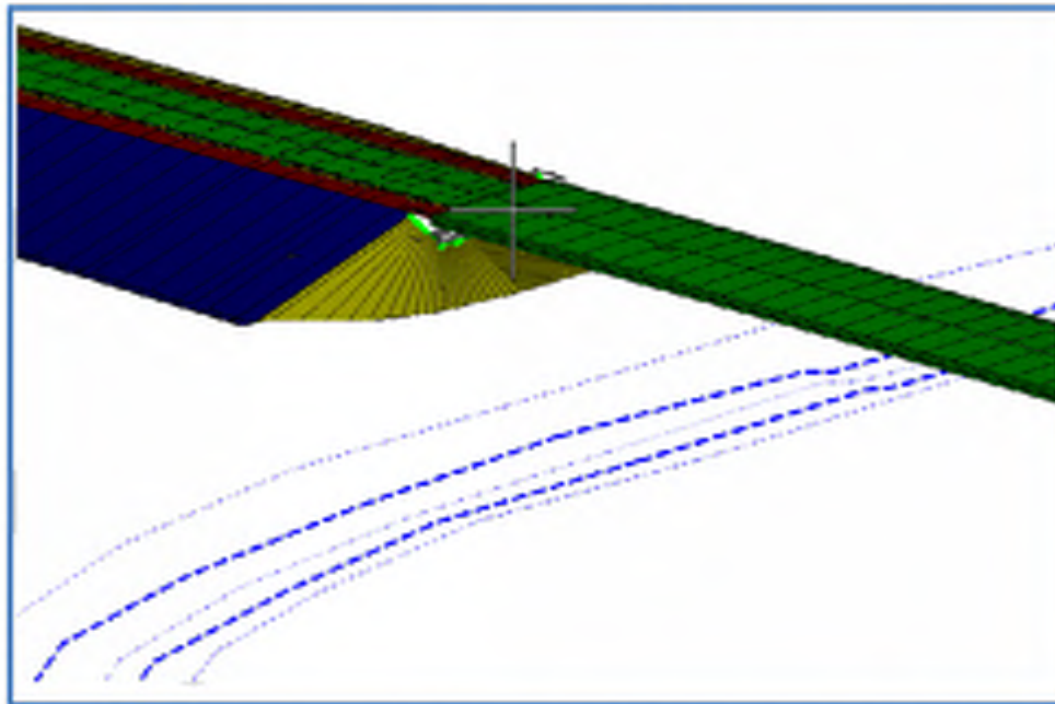
Figure 5: Bridge endroll modelled in 3D. Note that the bridge itself is also shown in this model, which is not required.
