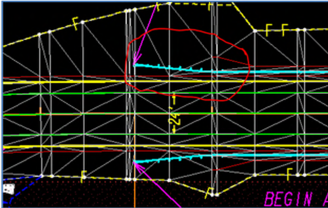
Figure 4: Overlaying the 2D DGN files with the triangulation from the 3D model shows that the 3D model triangles are not accounting for the guardrail terminal pod grading. The model should be updated to account for this grading, which will affect construction limits.
